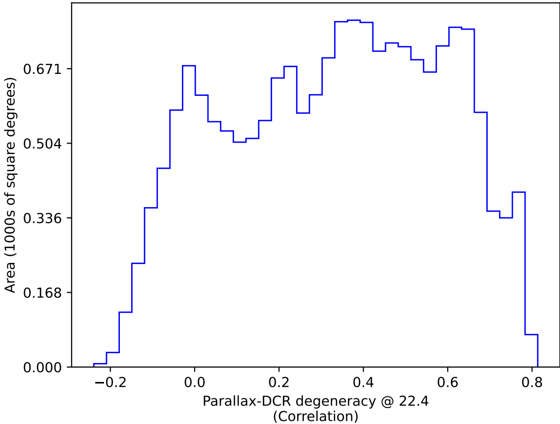
too_ignore_10_4v3.4_10yrs WFD: Parallax-DCR degeneracy @ 22.4
