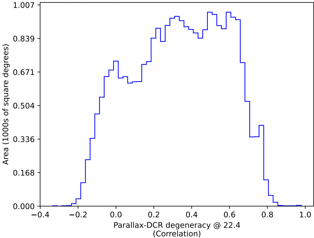
too_ignore_10_4v3.4_10yrs All sky: Parallax-DCR degeneracy @ 22.4
