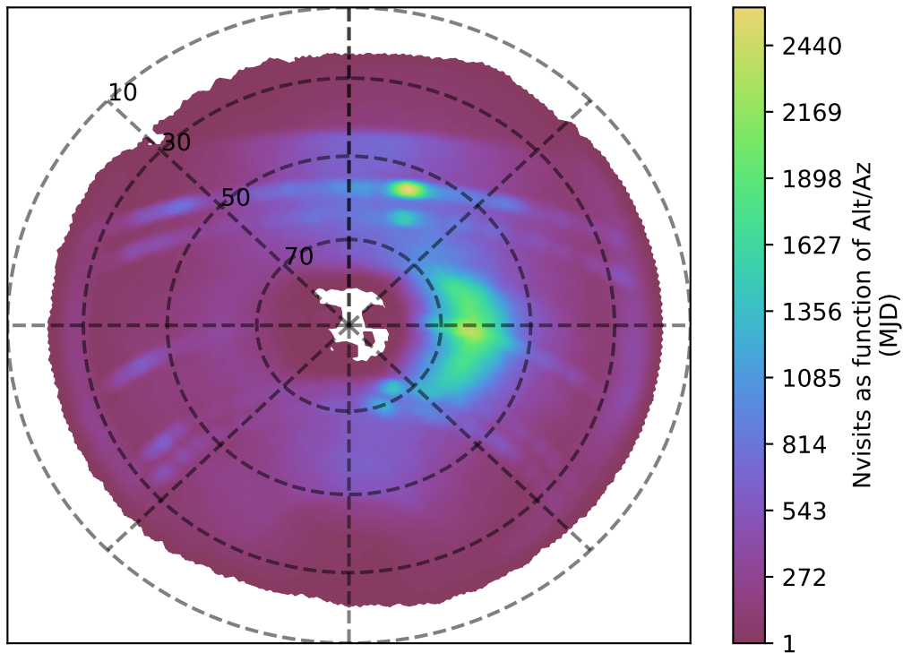
too_ignore_10_4v3.4_10yrs z band: Nvisits as function of Alt/Az
