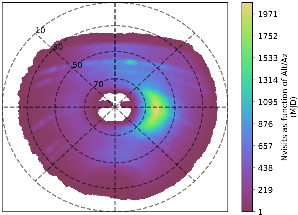
too_ignore_10_4v3.4_10yrs y band: Nvisits as function of Alt/Az
