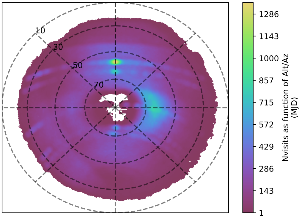
too_ignore_10_4v3.4_10yrs g band: Nvisits as function of Alt/Az
