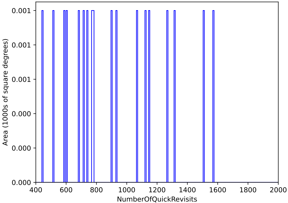
too_ignore_10_4v3.4_10yrs WFD: NumberOfQuickRevisits
