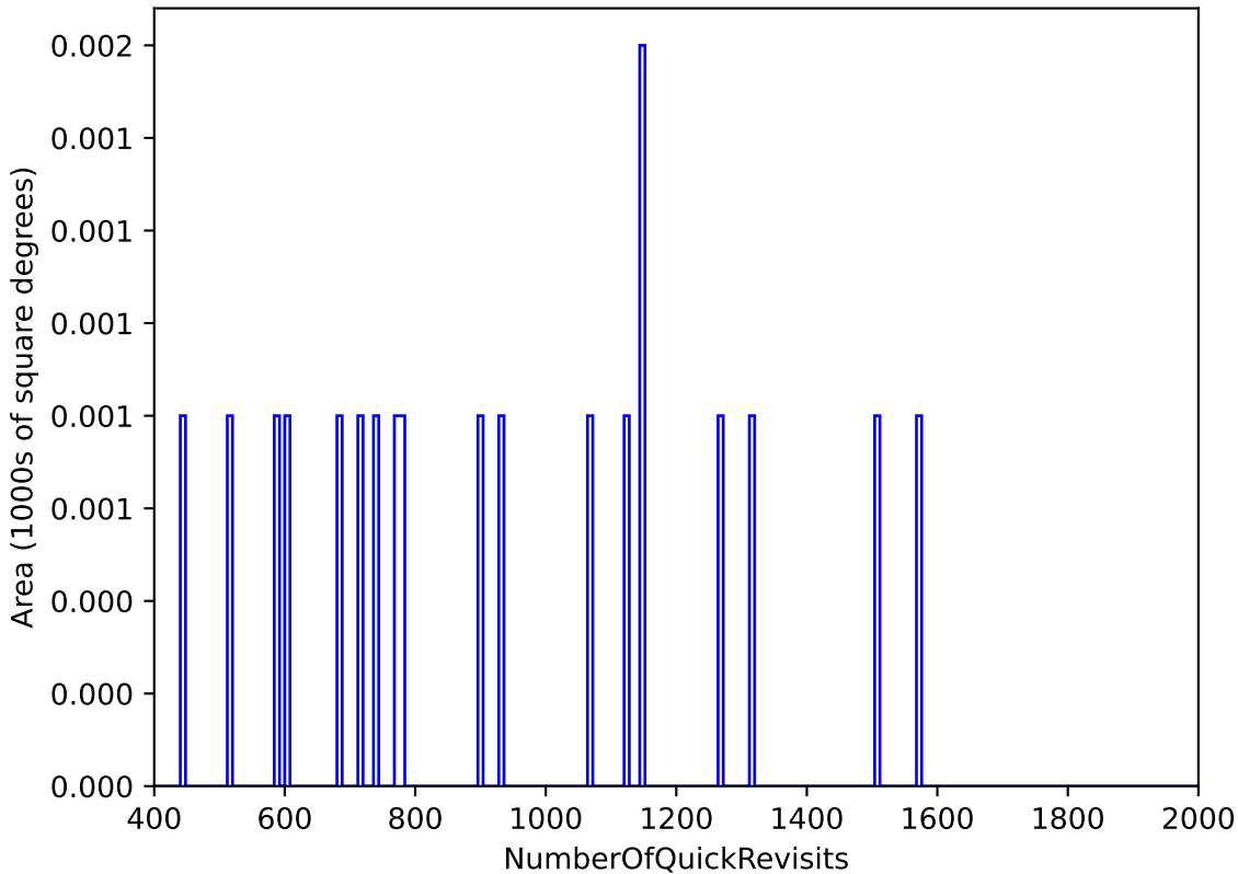
too_ignore_10_4v3.4_10yrs All sky: NumberOfQuickRevisits
