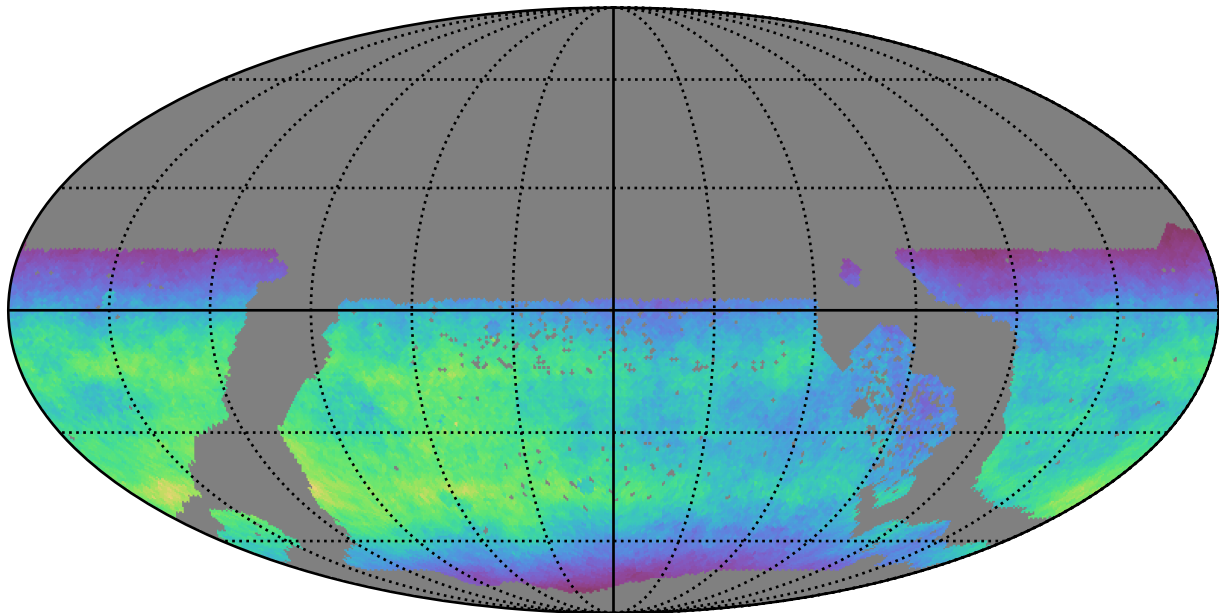
too_ignore_10_4v3.4_10yrs WFD y band: Normalized Teff
