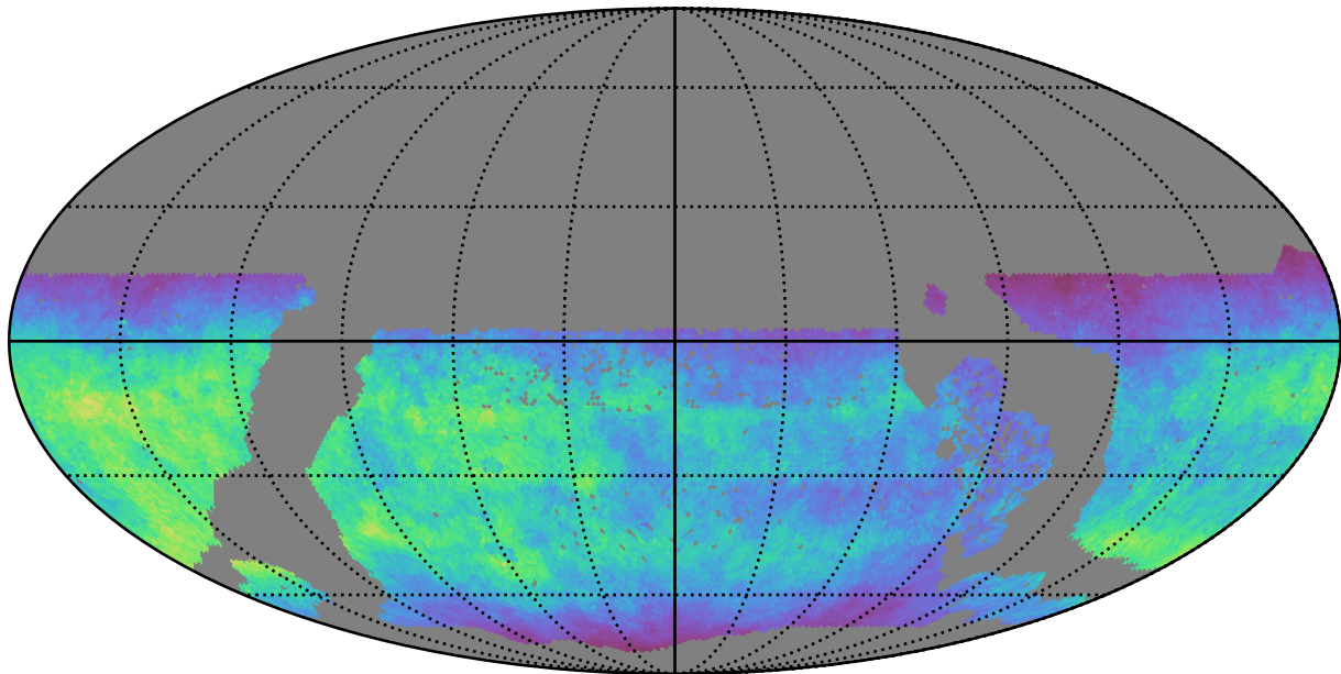
too_ignore_10_4v3.4_10yrs WFD u band: Normalized Teff
