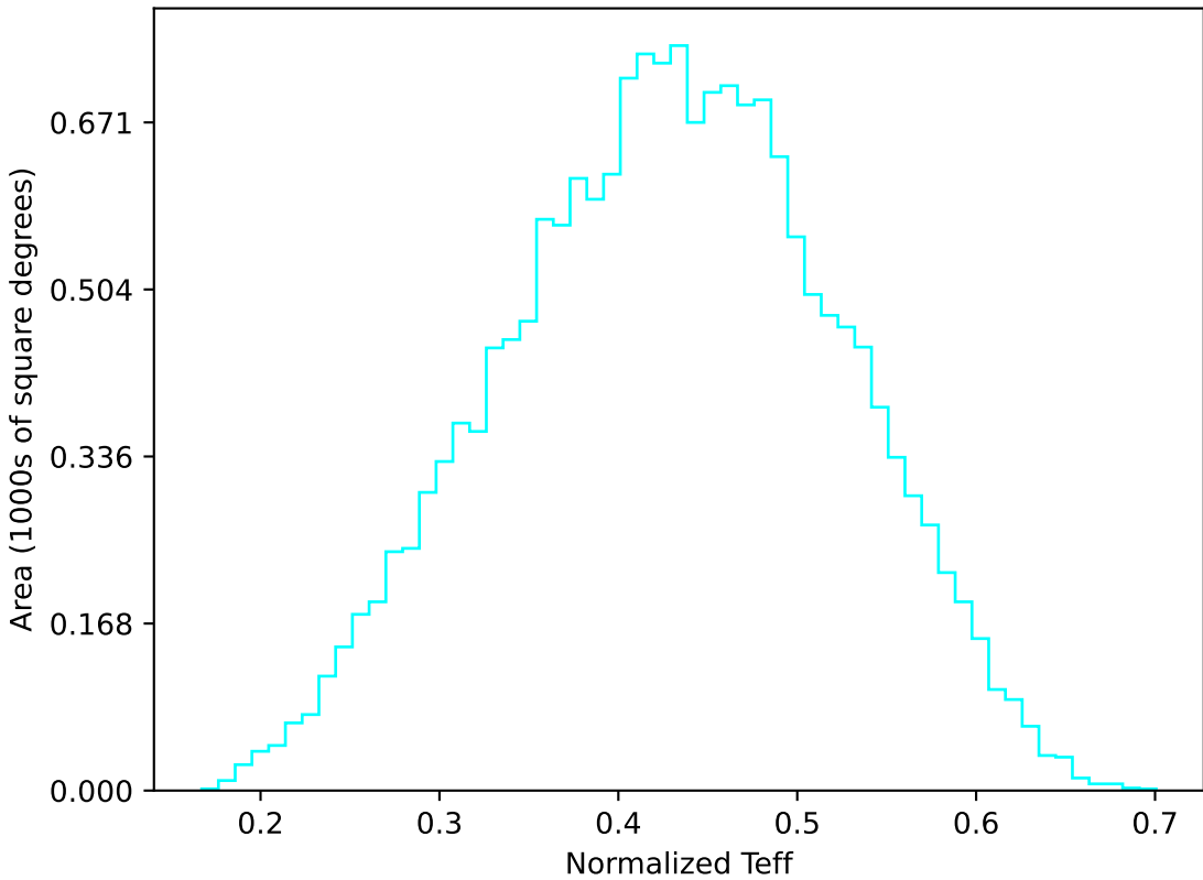
too_ignore_10_4v3.4_10yrs WFD u band: Normalized Teff
