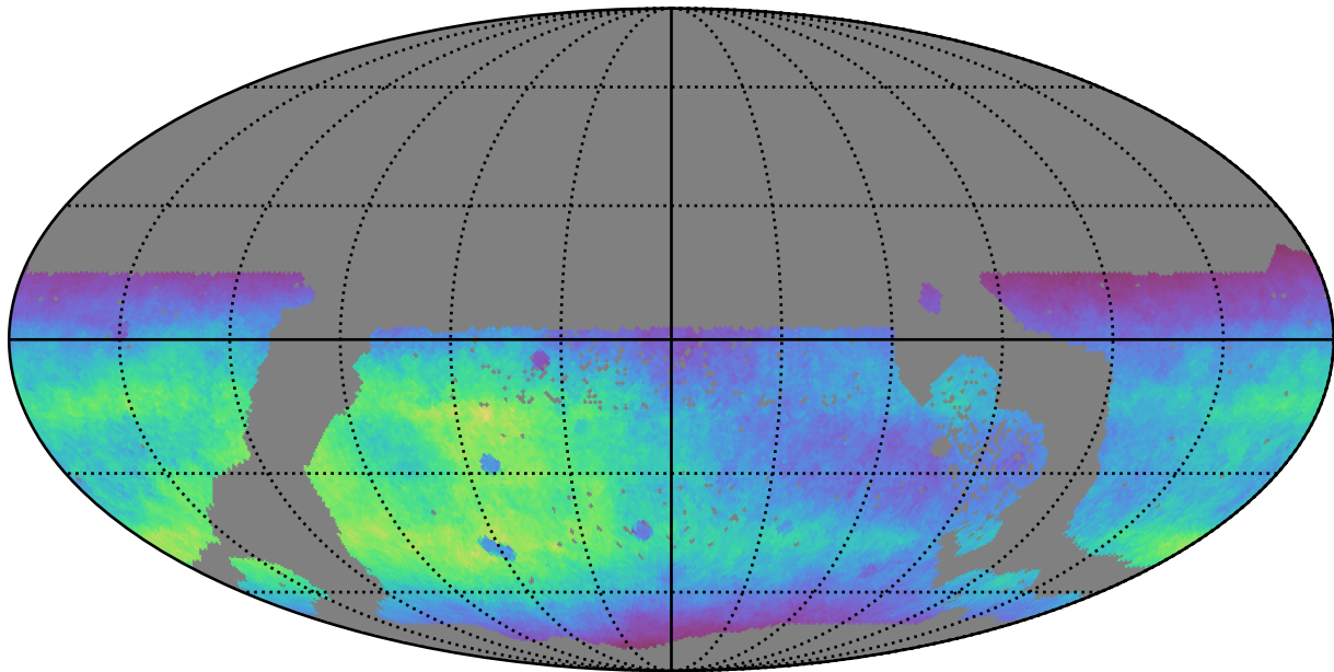
too_ignore_10_4v3.4_10yrs WFD r band: Normalized Teff
