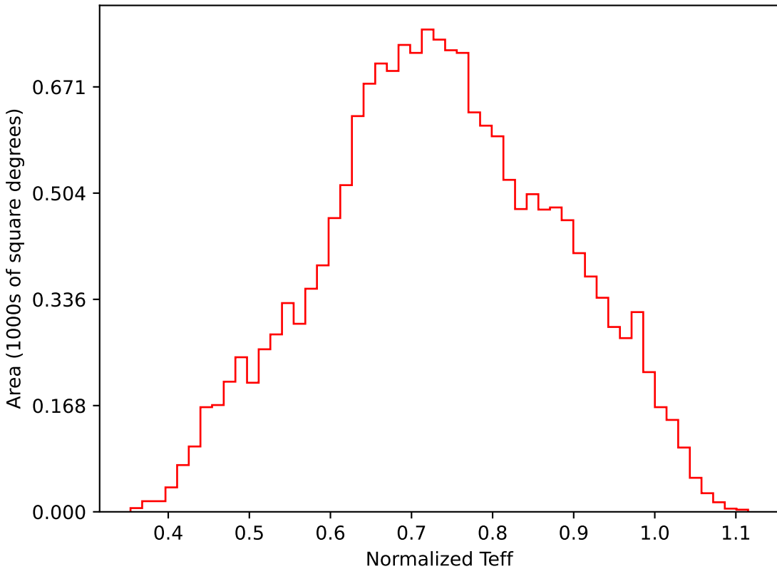
too_ignore_10_4v3.4_10yrs WFD i band: Normalized Teff
