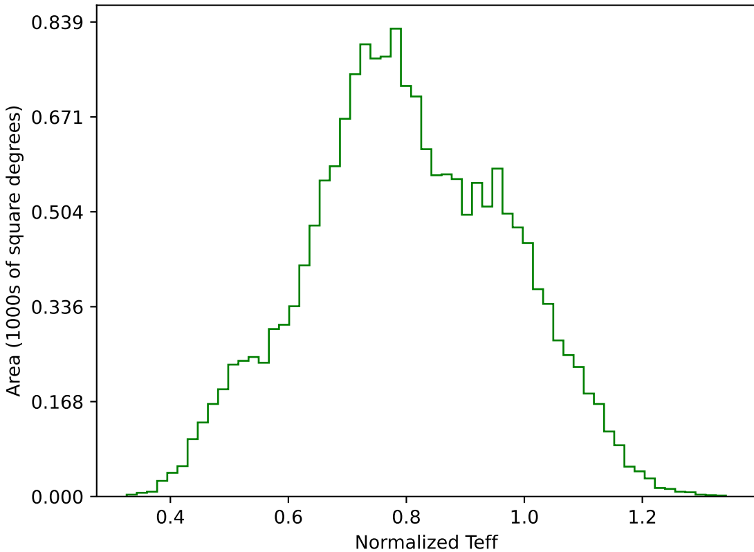
too_ignore_10_4v3.4_10yrs WFD g band: Normalized Teff
