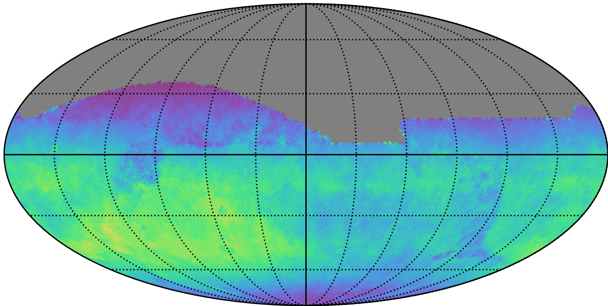
too_ignore_10_4v3.4_10yrs All sky z band: Normalized Teff
