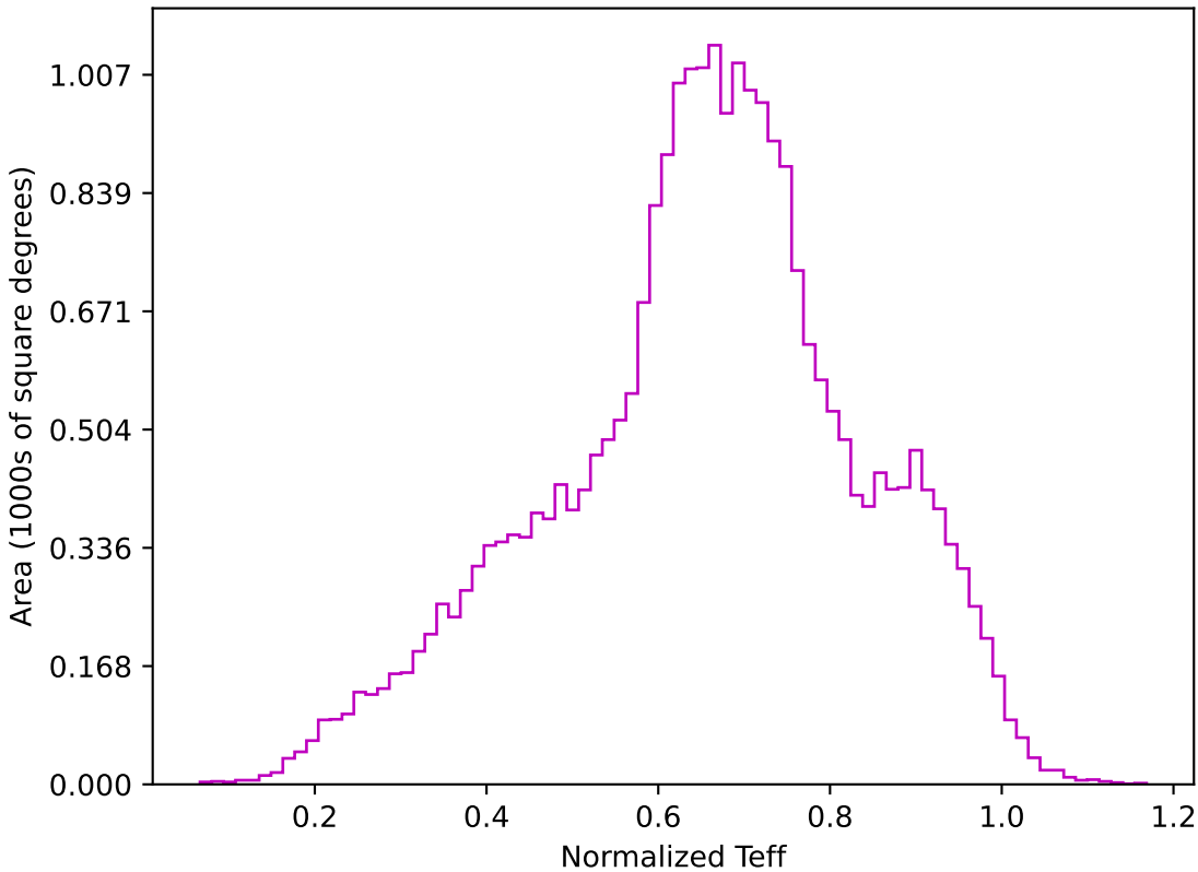
too_ignore_10_4v3.4_10yrs All sky z band: Normalized Teff
