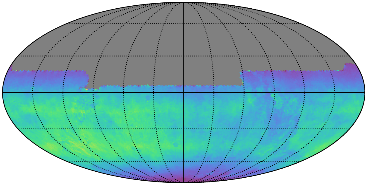
too_ignore_10_4v3.4_10yrs All sky y band: Normalized Teff
