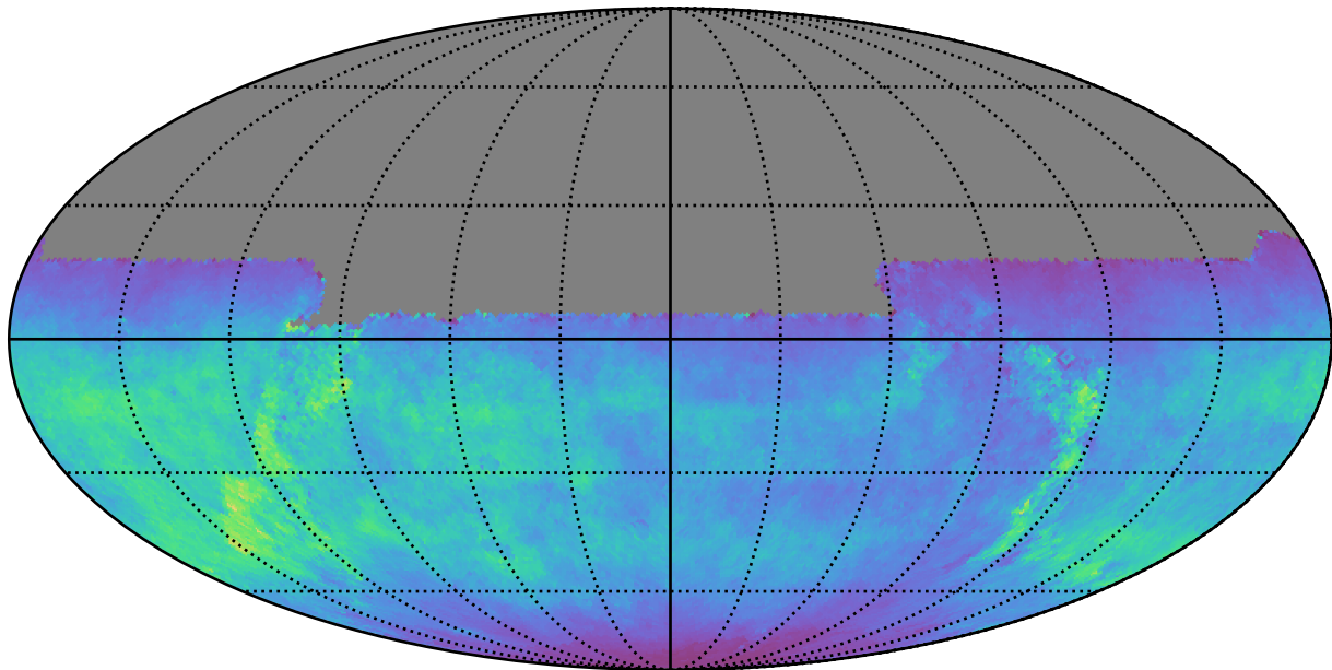
too_ignore_10_4v3.4_10yrs All sky u band: Normalized Teff
