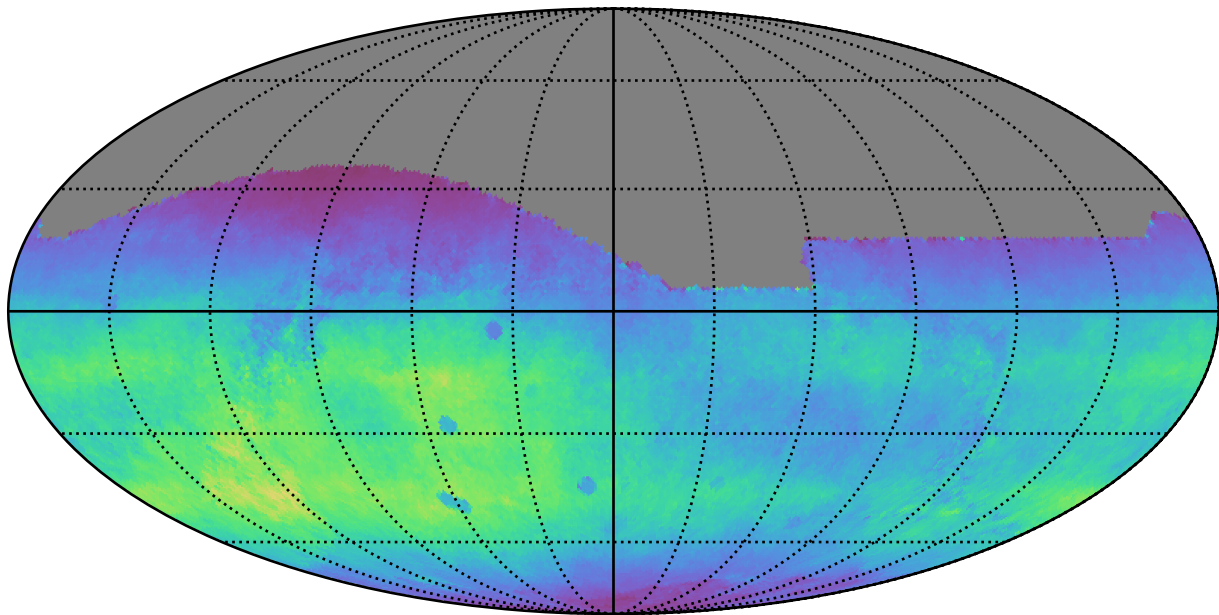
too_ignore_10_4v3.4_10yrs All sky r band: Normalized Teff
