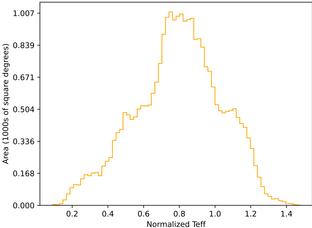
too_ignore_10_4v3.4_10yrs All sky r band: Normalized Teff
