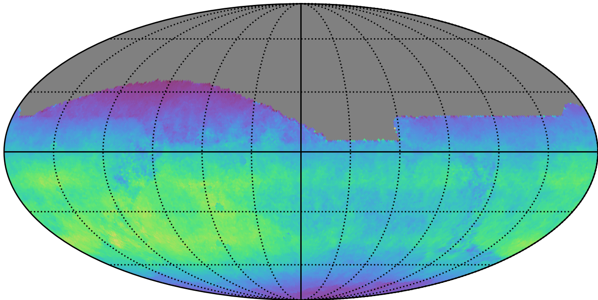
too_ignore_10_4v3.4_10yrs All sky i band: Normalized Teff
