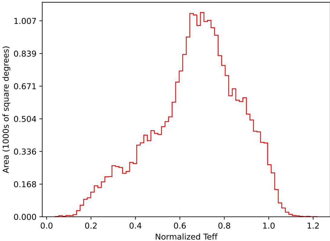
too_ignore_10_4v3.4_10yrs All sky i band: Normalized Teff
