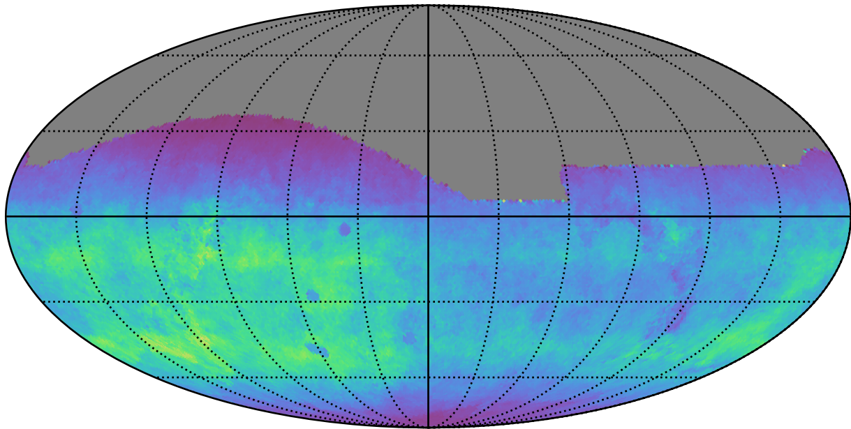
too_ignore_10_4v3.4_10yrs All sky g band: Normalized Teff
