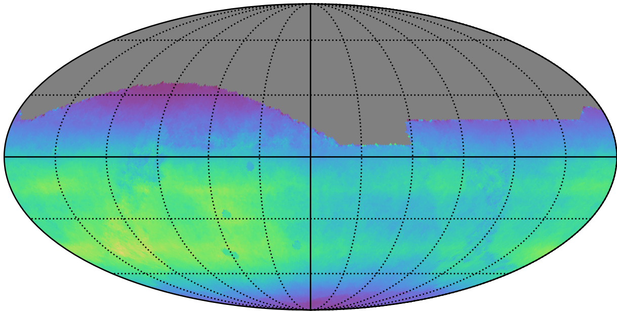
too_ignore_10_4v3.4_10yrs All sky all bands: Normalized Teff
