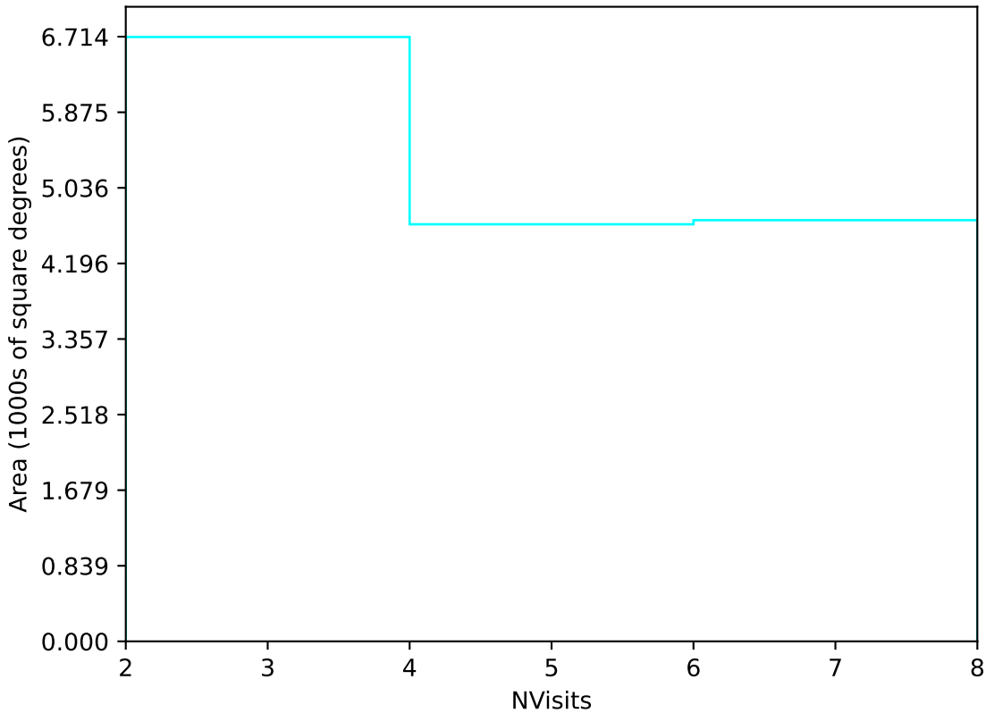
too_ignore_10_4v3.4_10yrs Yr 3-4 u band: NVisits
