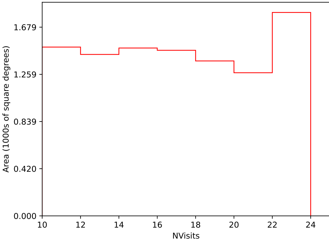
too_ignore_10_4v3.4_10yrs Yr 3-4 i band: NVisits
