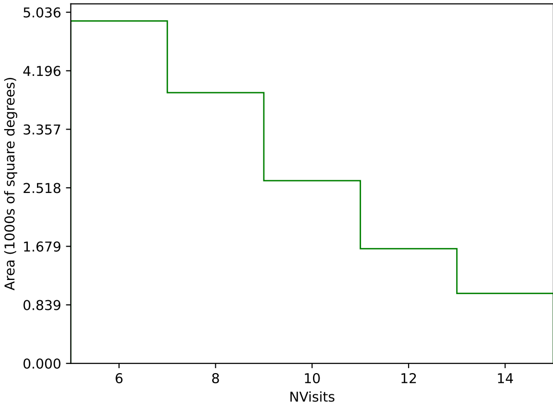
too_ignore_10_4v3.4_10yrs Yr 3-4 g band: NVisits
