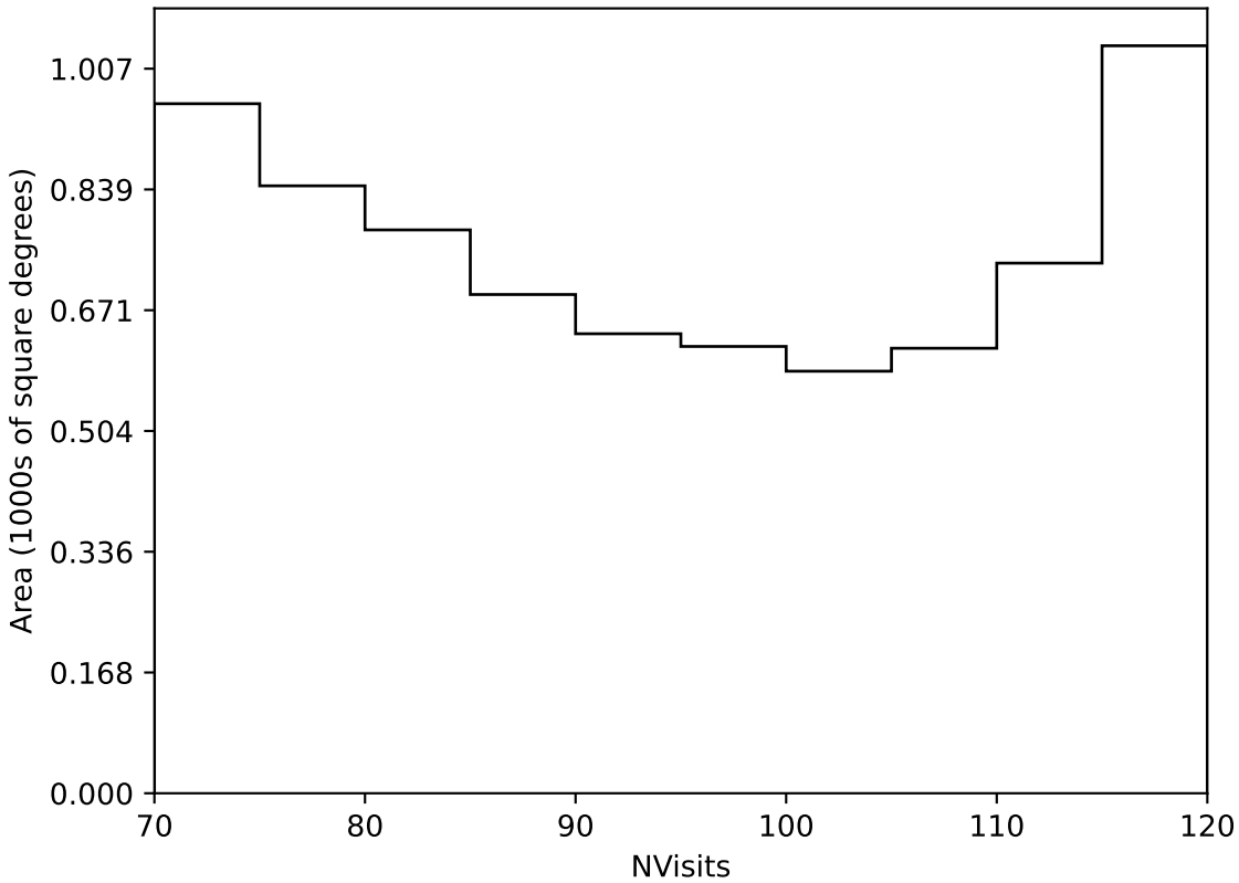
too_ignore_10_4v3.4_10yrs Yr 3-4 all bands: NVisits
