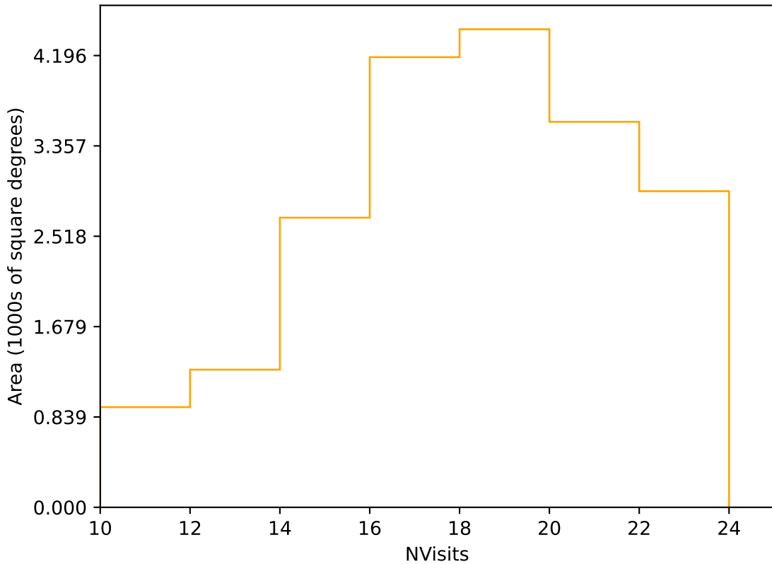
too_ignore_10_4v3.4_10yrs Yr 1 r band: NVisits
