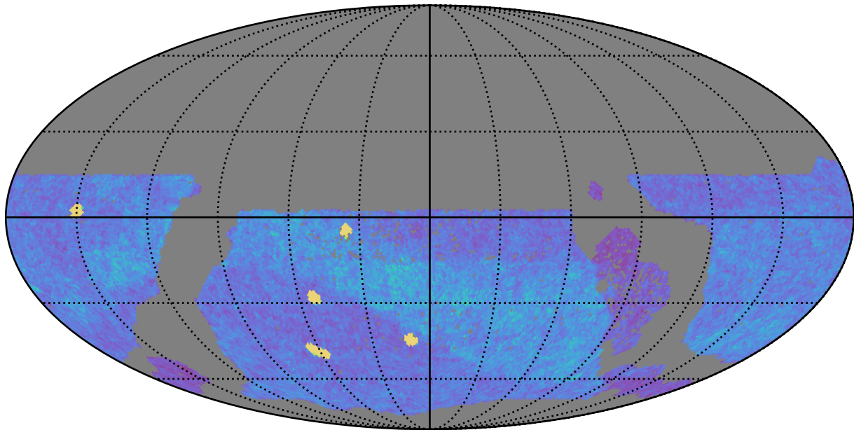
too_ignore_10_4v3.4_10yrs WFD z band: NVisits
