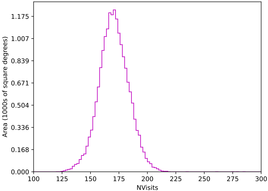
too_ignore_10_4v3.4_10yrs WFD z band: NVisits
