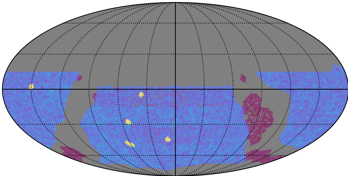
too_ignore_10_4v3.4_10yrs WFD y band: NVisits
