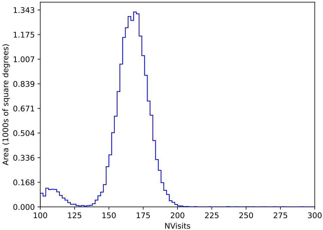
too_ignore_10_4v3.4_10yrs WFD y band: NVisits
