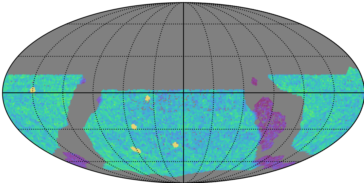
too_ignore_10_4v3.4_10yrs WFD u band: NVisits
