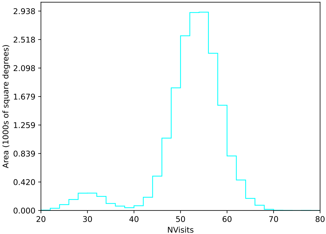
too_ignore_10_4v3.4_10yrs WFD u band: NVisits
