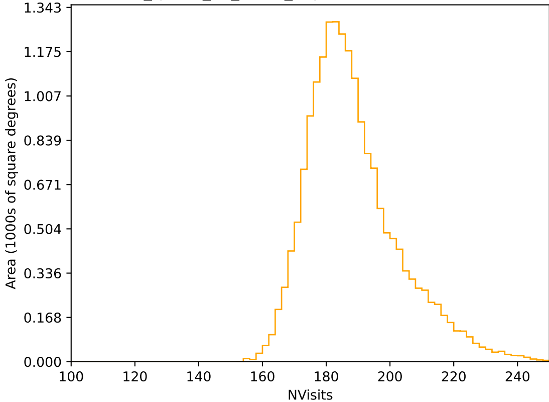
too_ignore_10_4v3.4_10yrs WFD r band: NVisits
