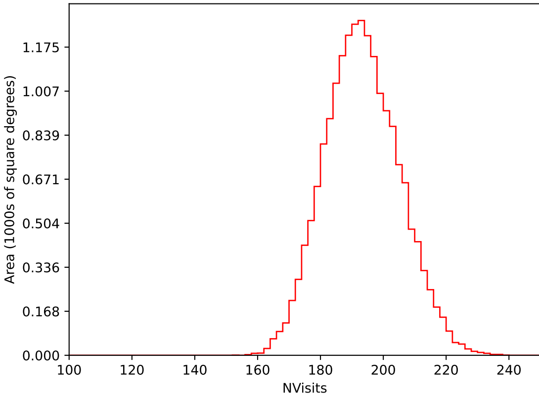
too_ignore_10_4v3.4_10yrs WFD i band: NVisits
