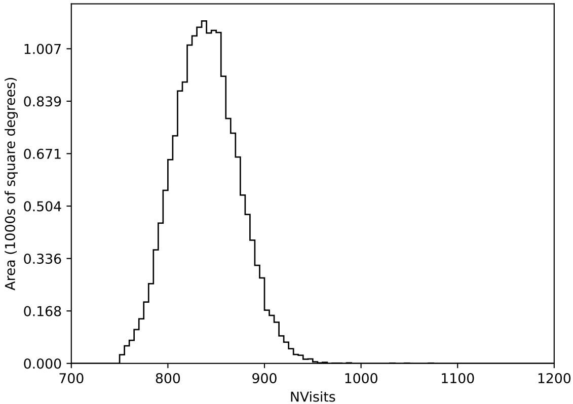
too_ignore_10_4v3.4_10yrs WFD all bands: NVisits
