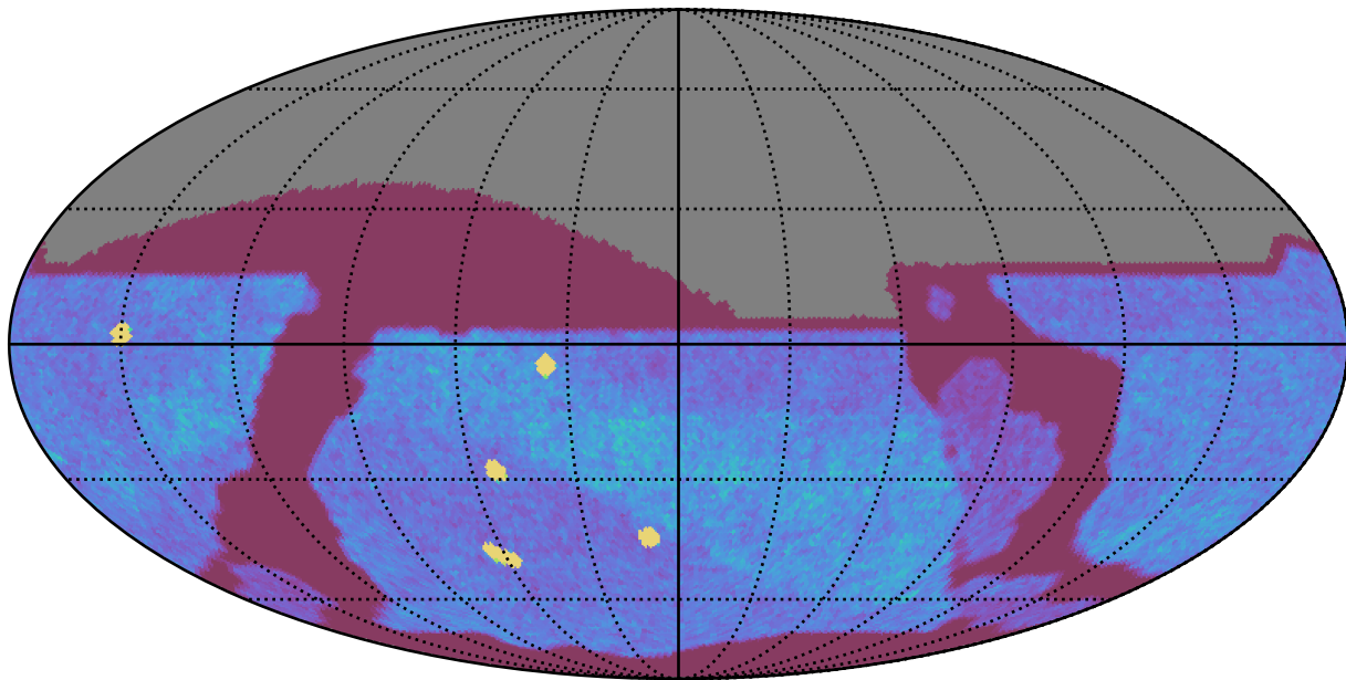
too_ignore_10_4v3.4_10yrs All sky z band: NVisits
