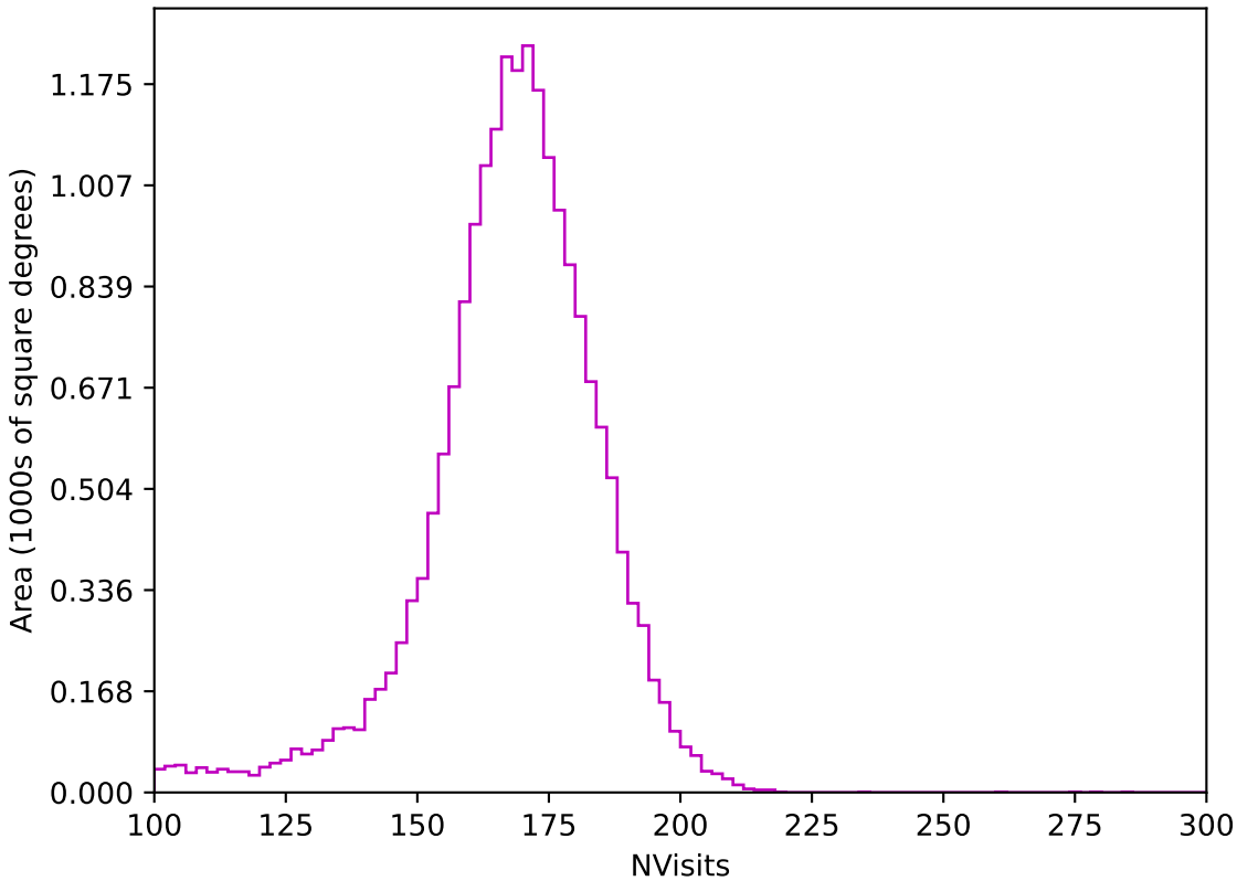
too_ignore_10_4v3.4_10yrs All sky z band: NVisits
