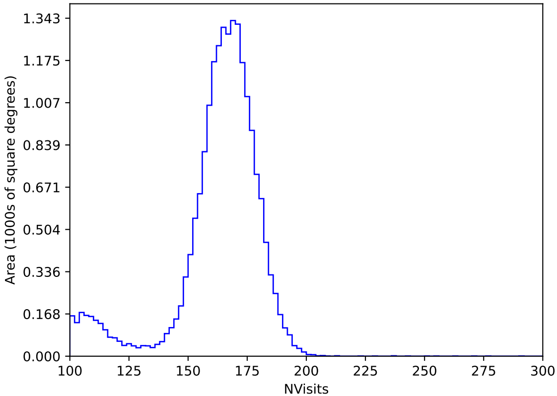
too_ignore_10_4v3.4_10yrs All sky y band: NVisits
