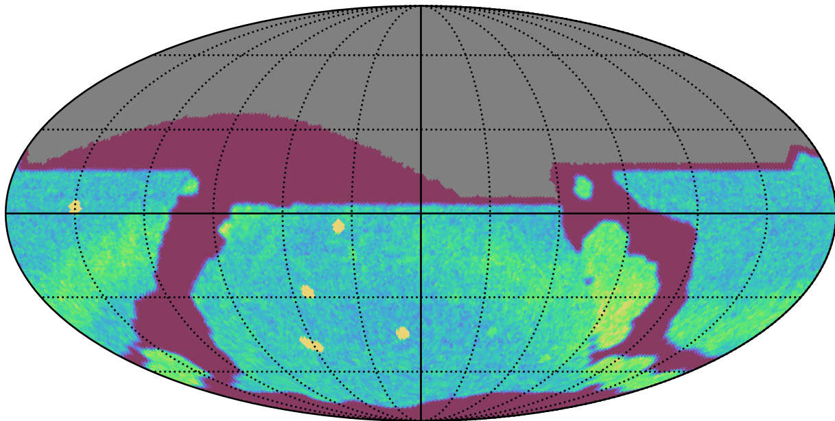
too_ignore_10_4v3.4_10yrs All sky r band: NVisits
