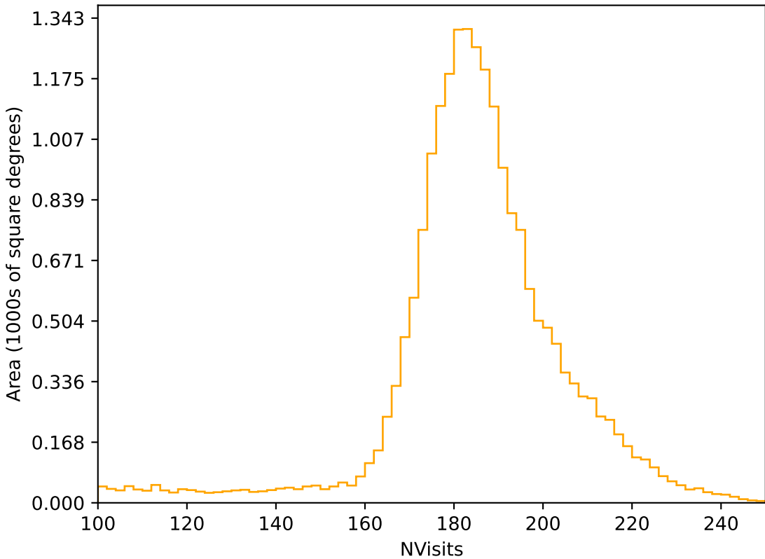
too_ignore_10_4v3.4_10yrs All sky r band: NVisits
