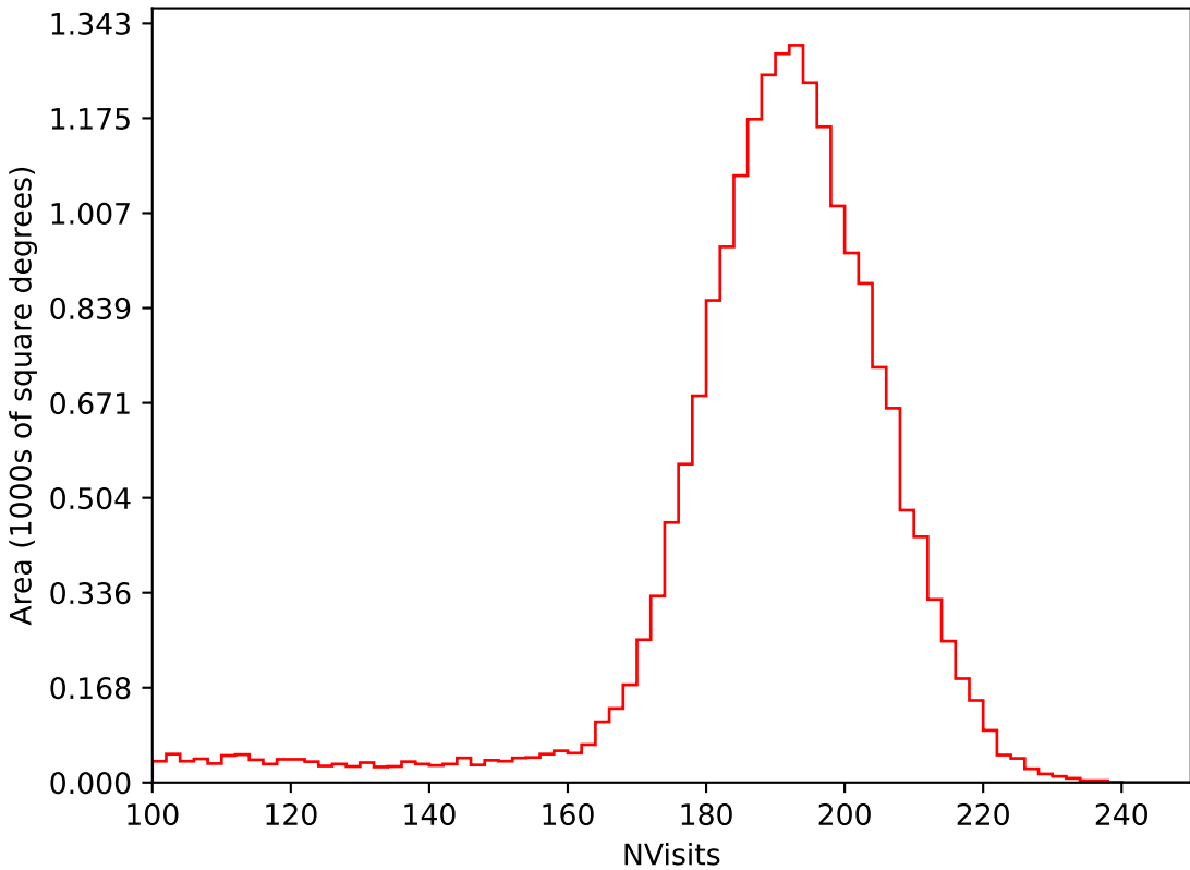
too_ignore_10_4v3.4_10yrs All sky i band: NVisits
