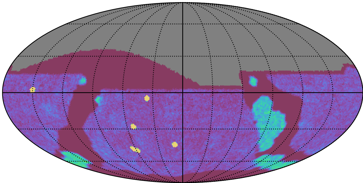
too_ignore_10_4v3.4_10yrs All sky g band: NVisits
