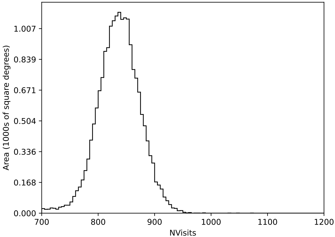
too_ignore_10_4v3.4_10yrs All sky all bands: NVisits
