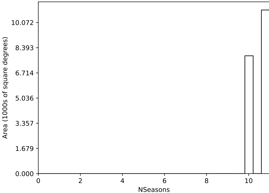
too_ignore_10_4v3.4_10yrs WFD all bands: NSeasons
