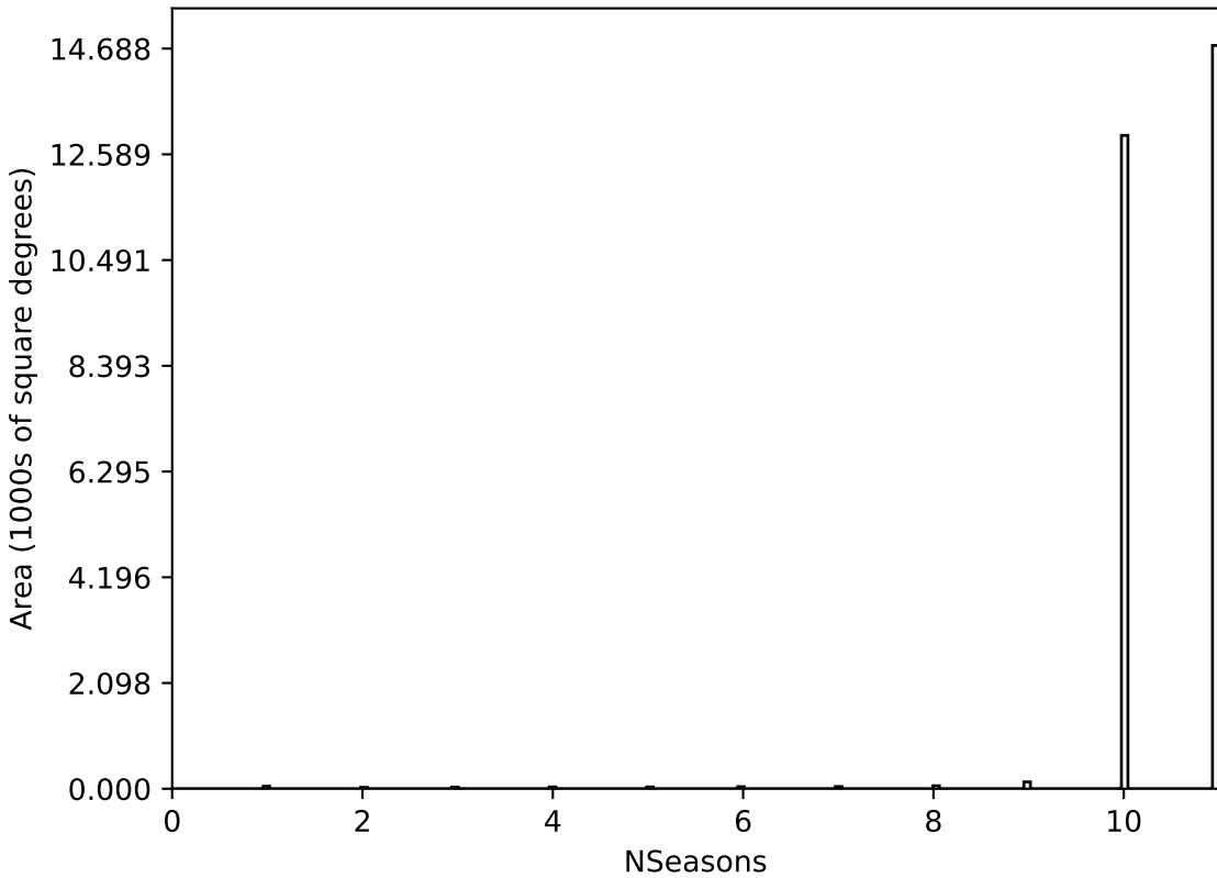
too_ignore_10_4v3.4_10yrs All sky all bands: NSeasons
