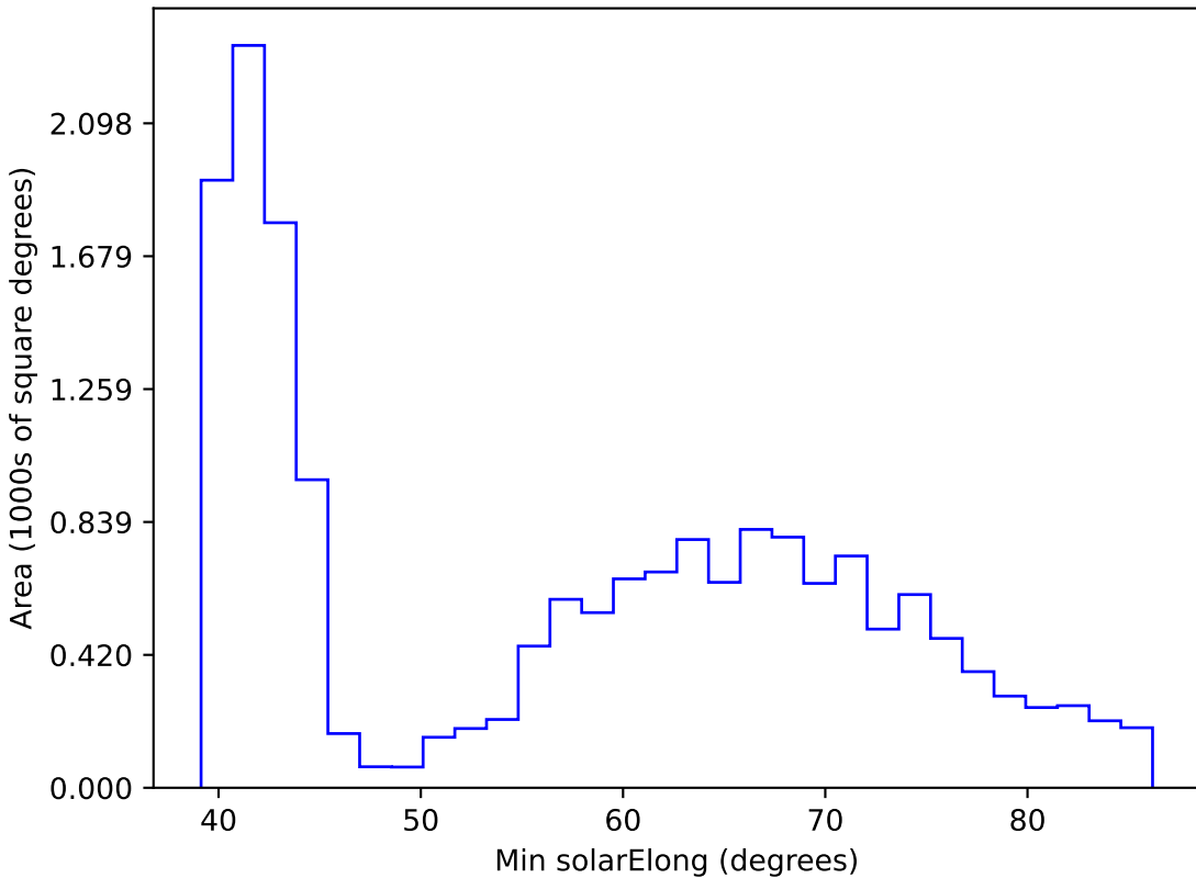
too_ignore_10_4v3.4_10yrs WFD r band: Min solarElong
