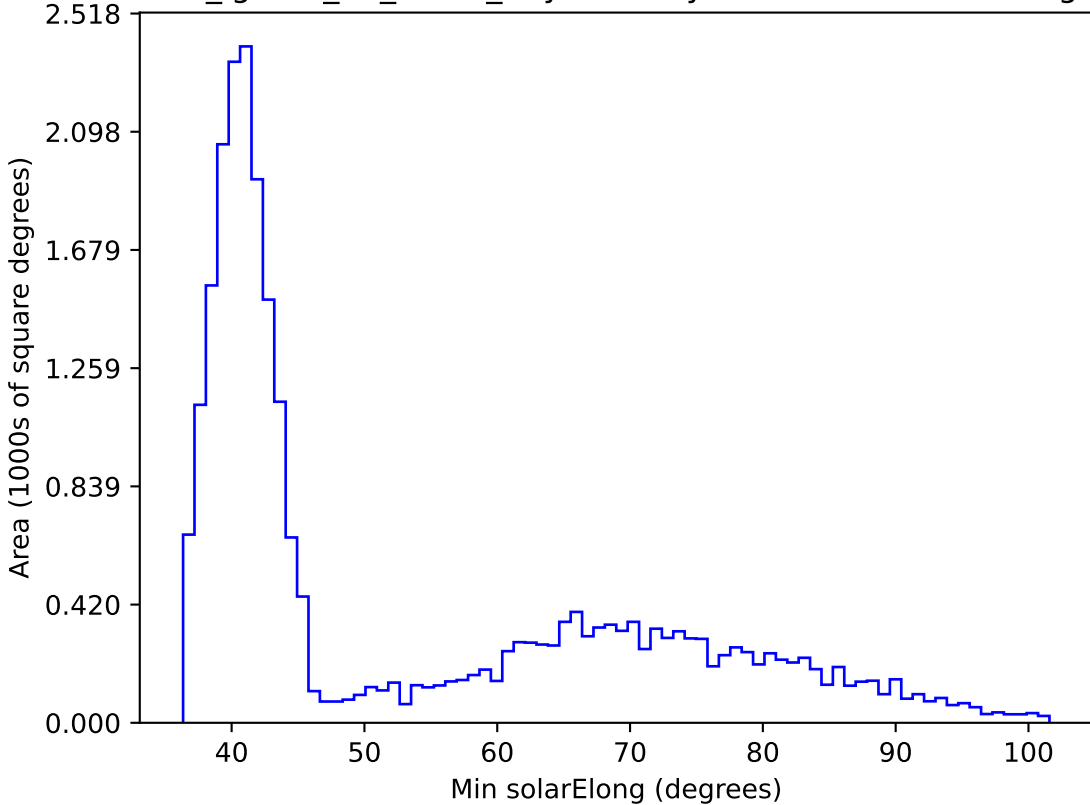
too_ignore_10_4v3.4_10yrs All sky z band: Min solarElong
