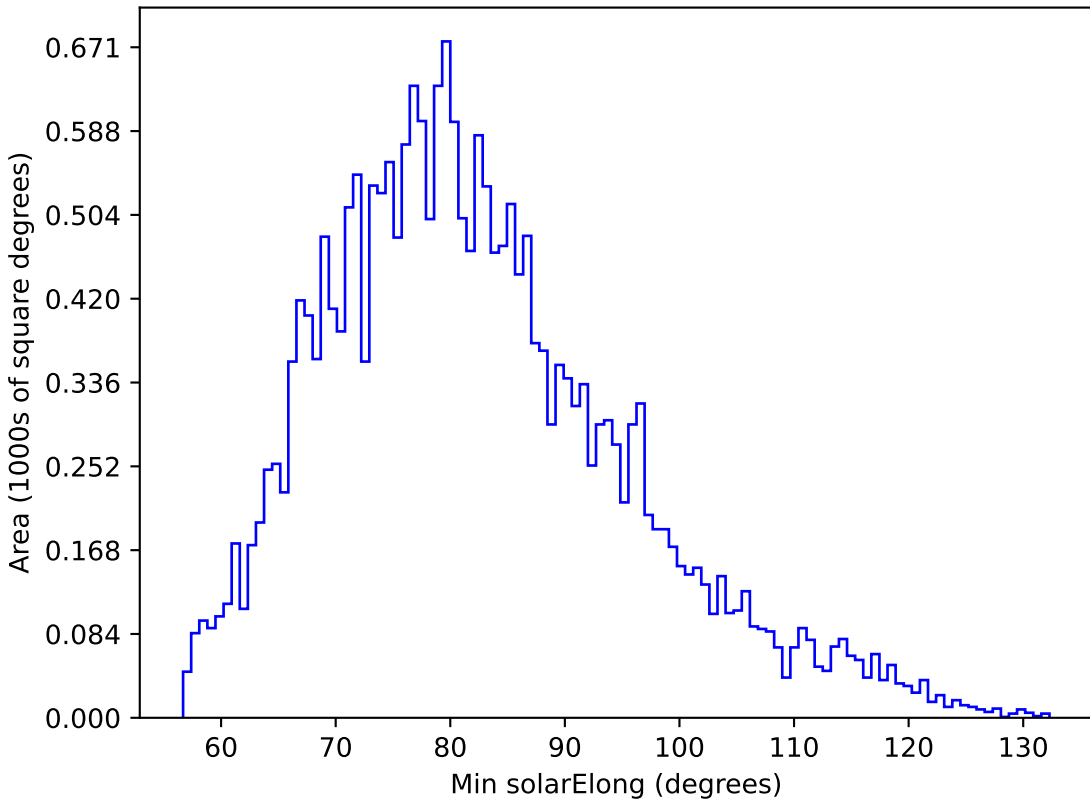
too_ignore_10_4v3.4_10yrs All sky u band: Min solarElong
